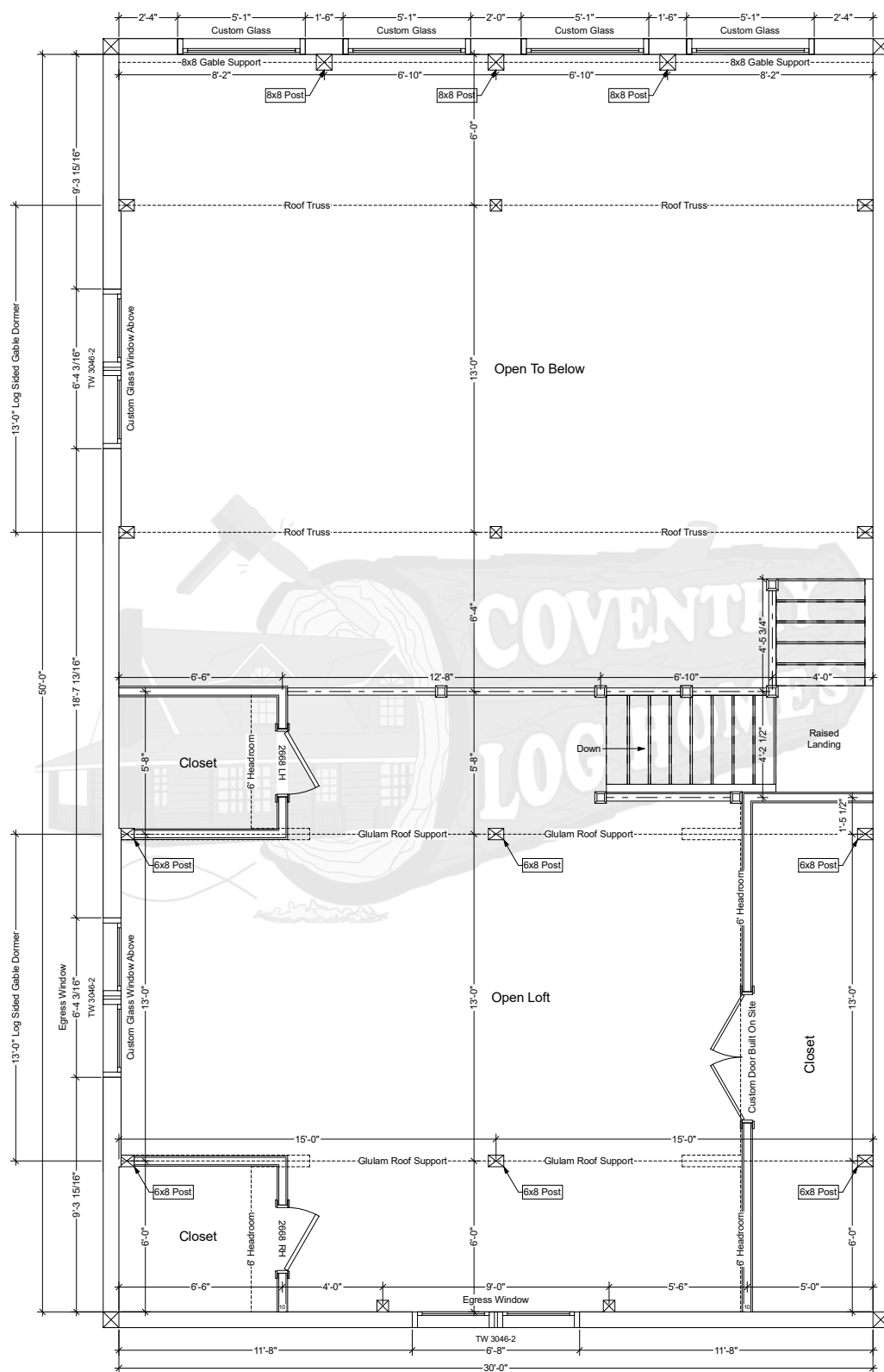
Boulder Second Floor Plan
