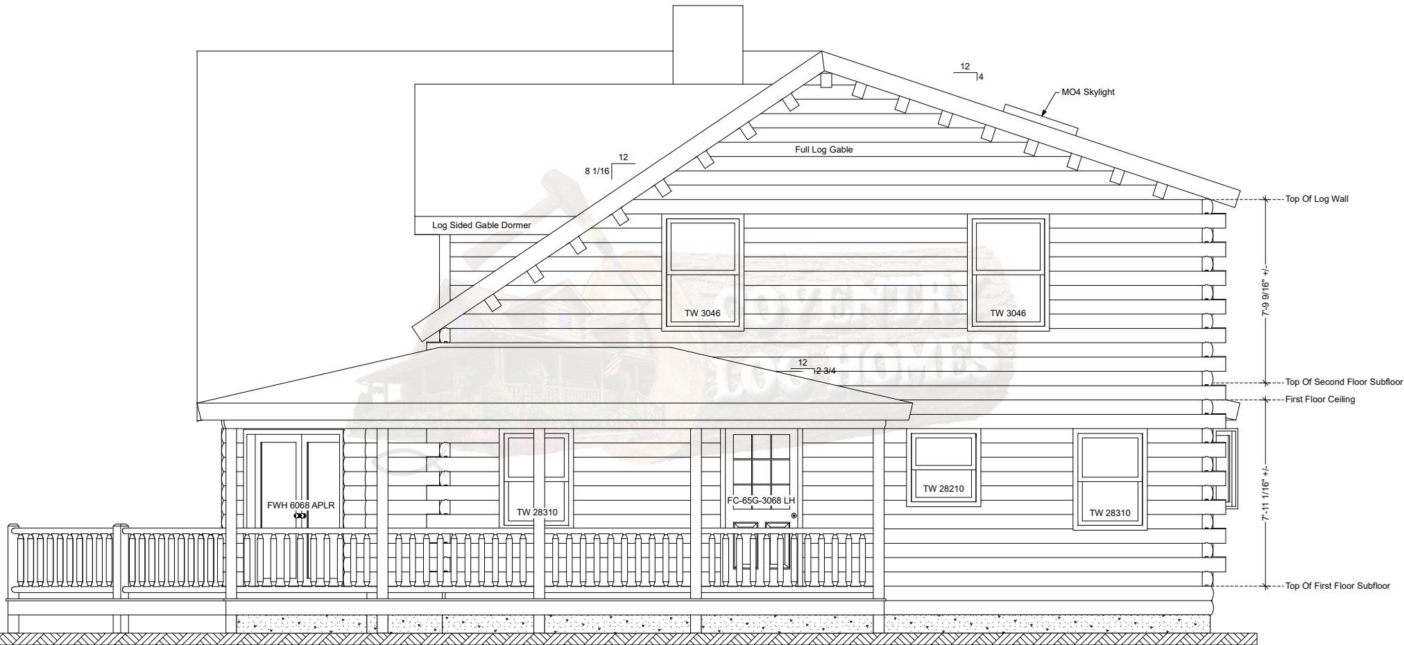
Bowman Right Elevation
