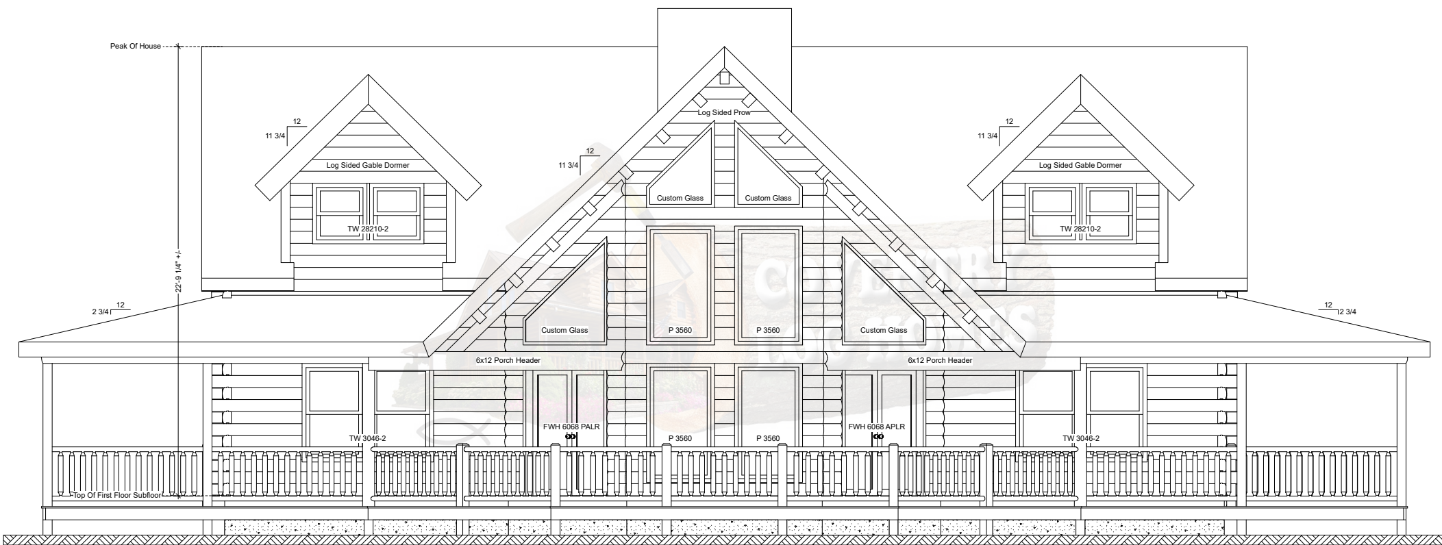
Bowman Front Elevation
