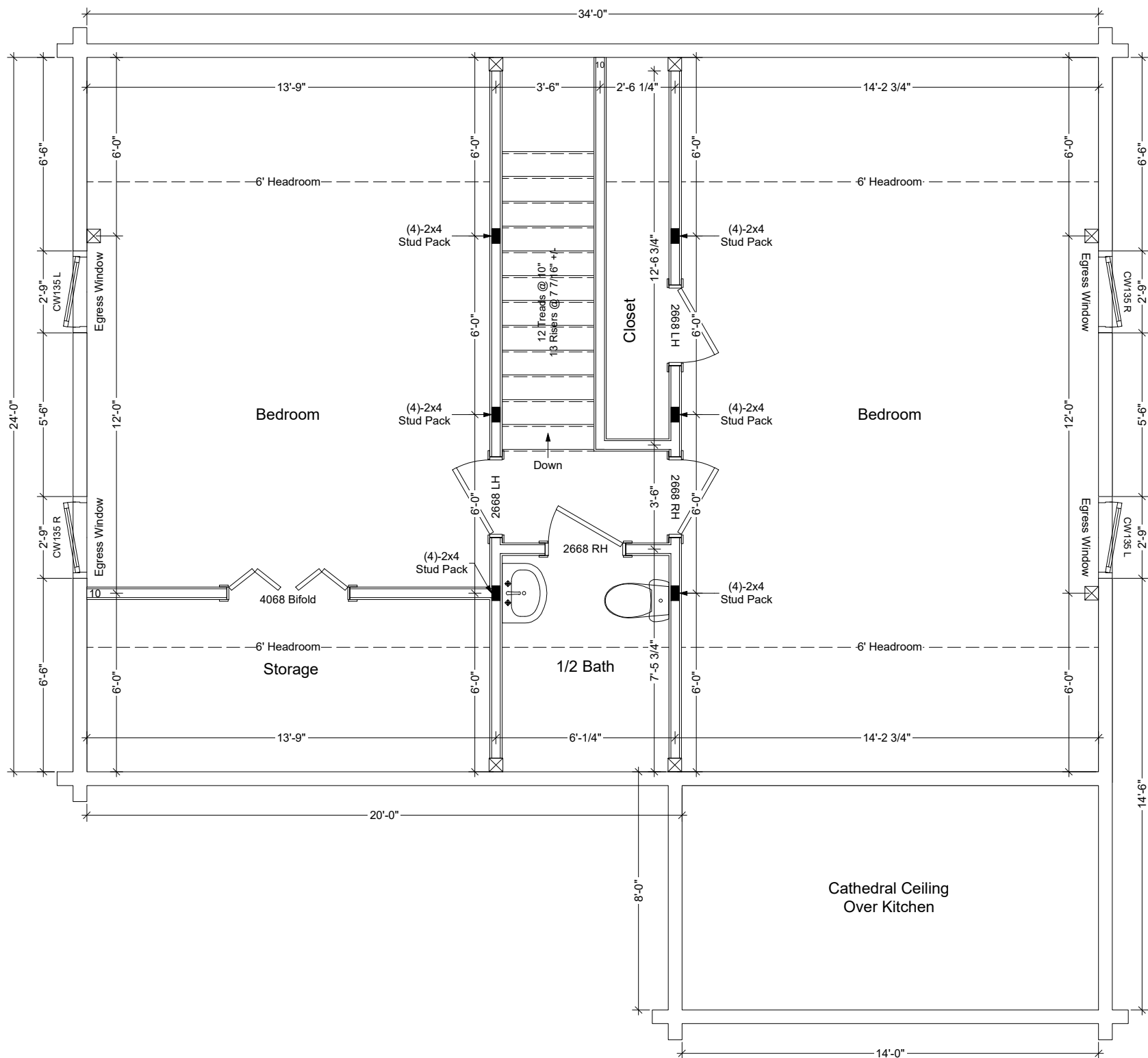
Greensboro Second Floor Plan
