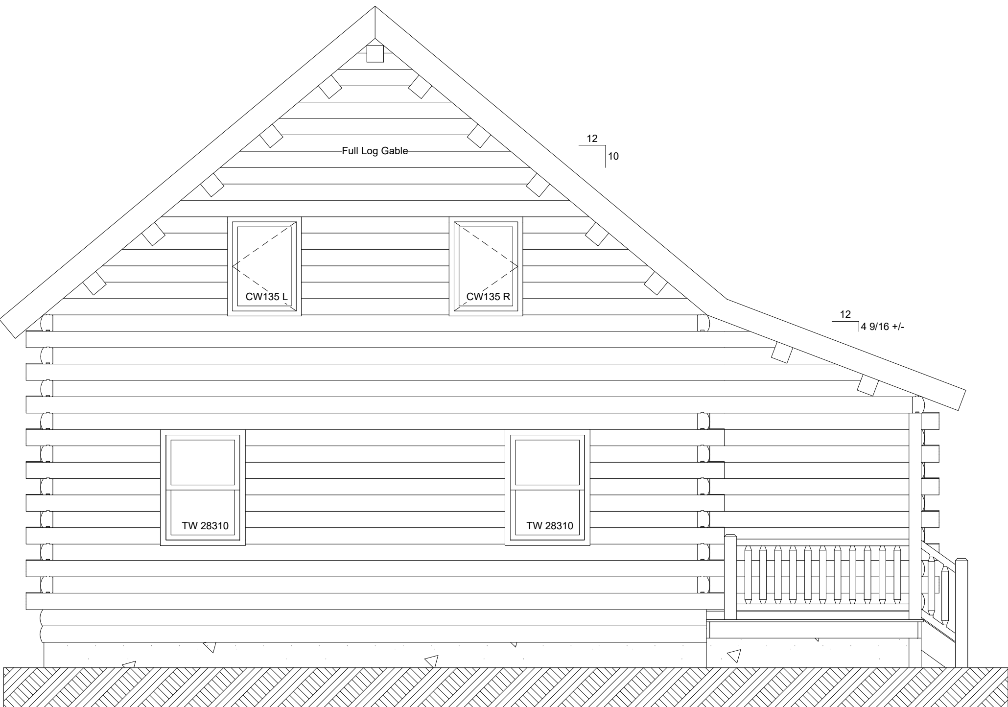
Greensboro Left Elevation
