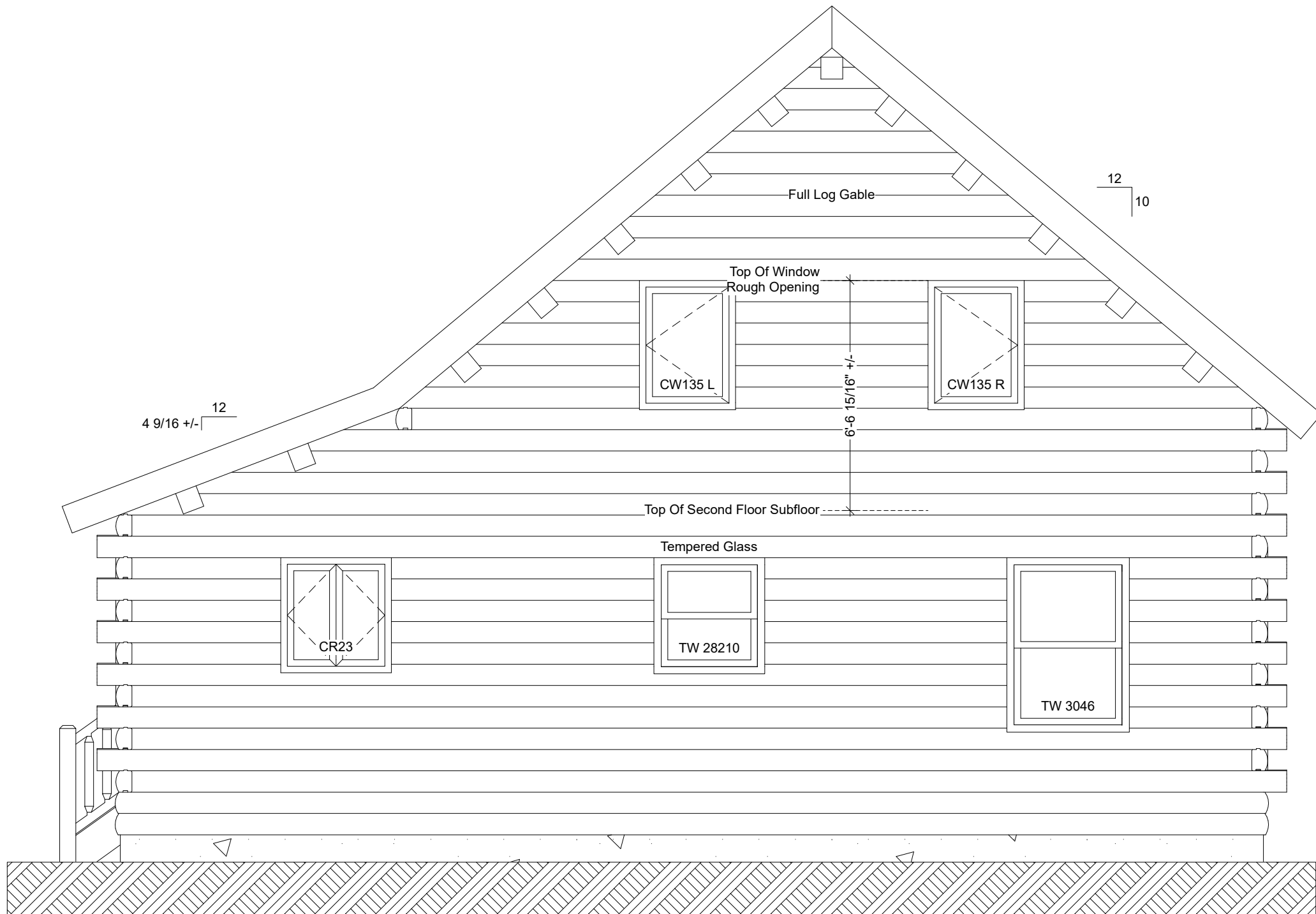
Greensboro Right Elevation
