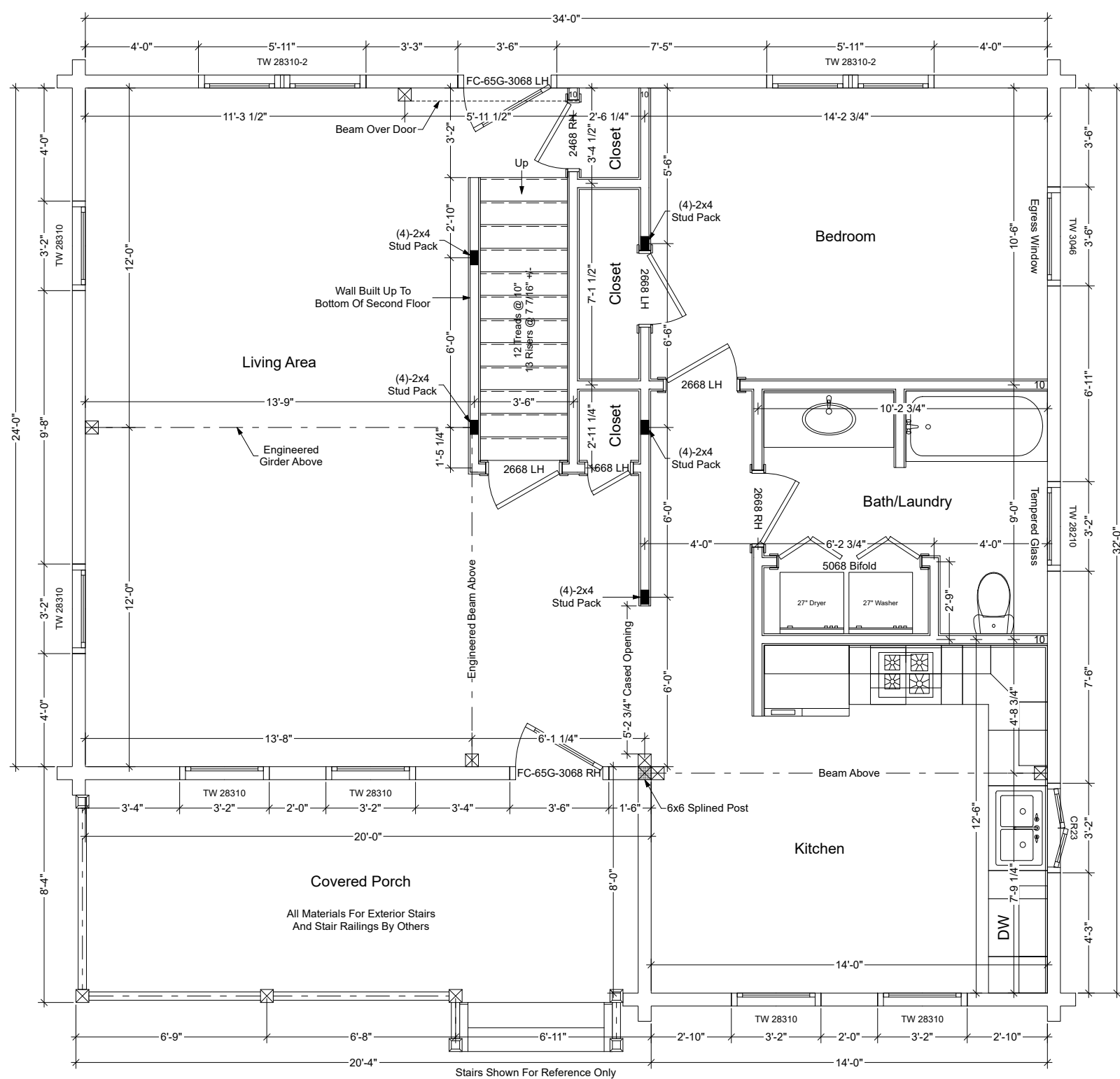
Greensboro First Floor Plan
