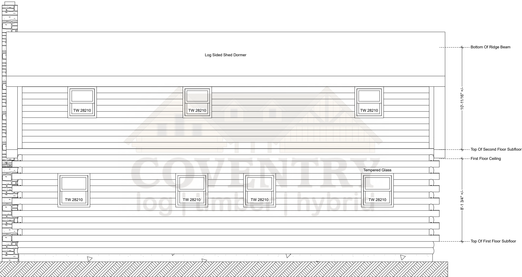
Wyoming Rear Elevation
