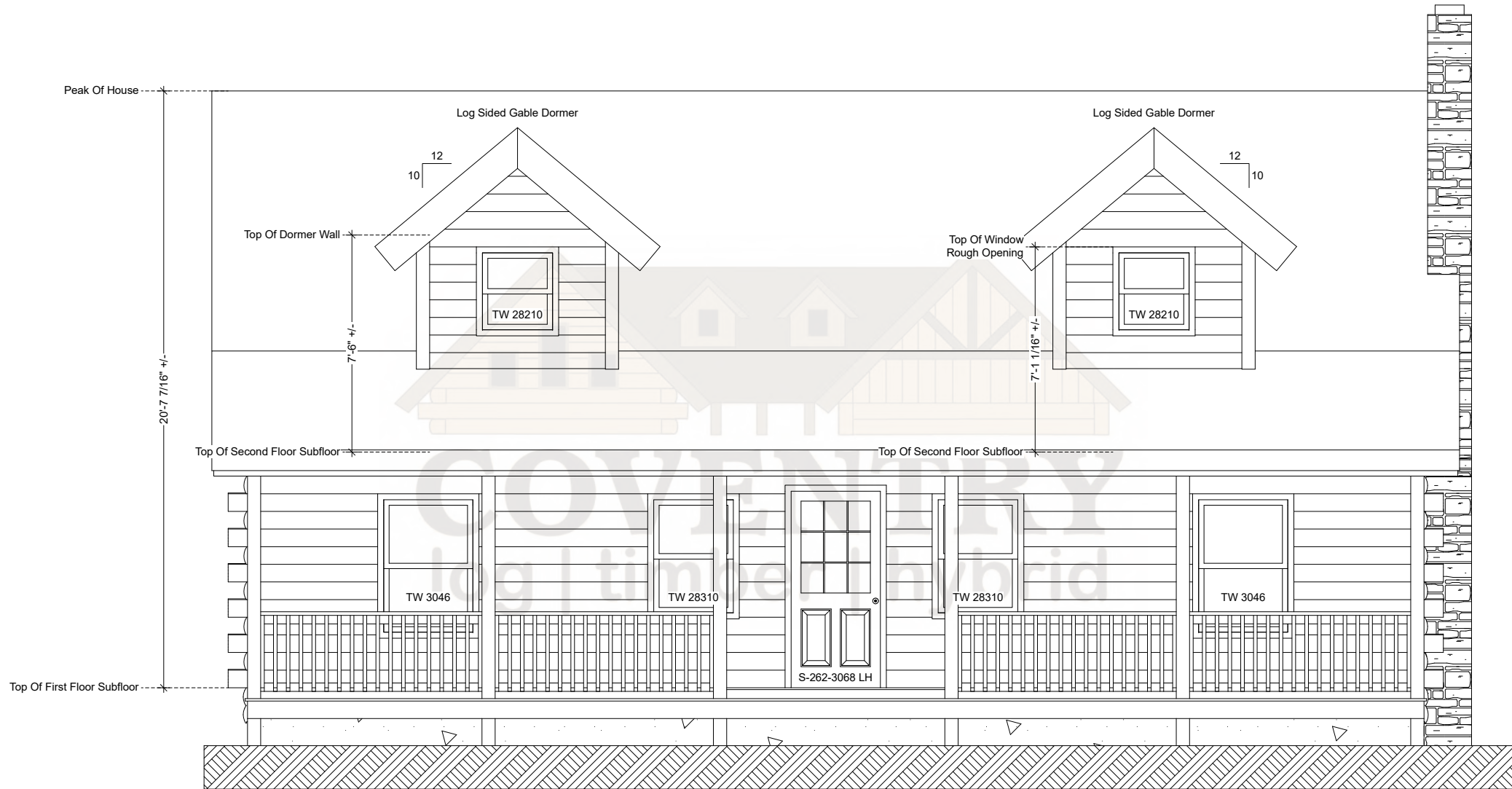
Wyoming Front Elevation
