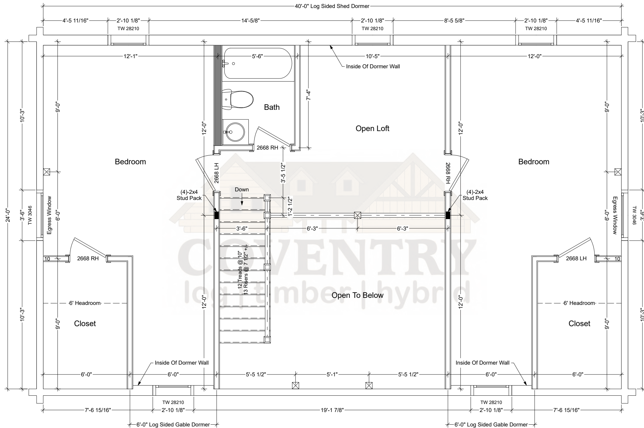
Wyoming Second Floor Plan
