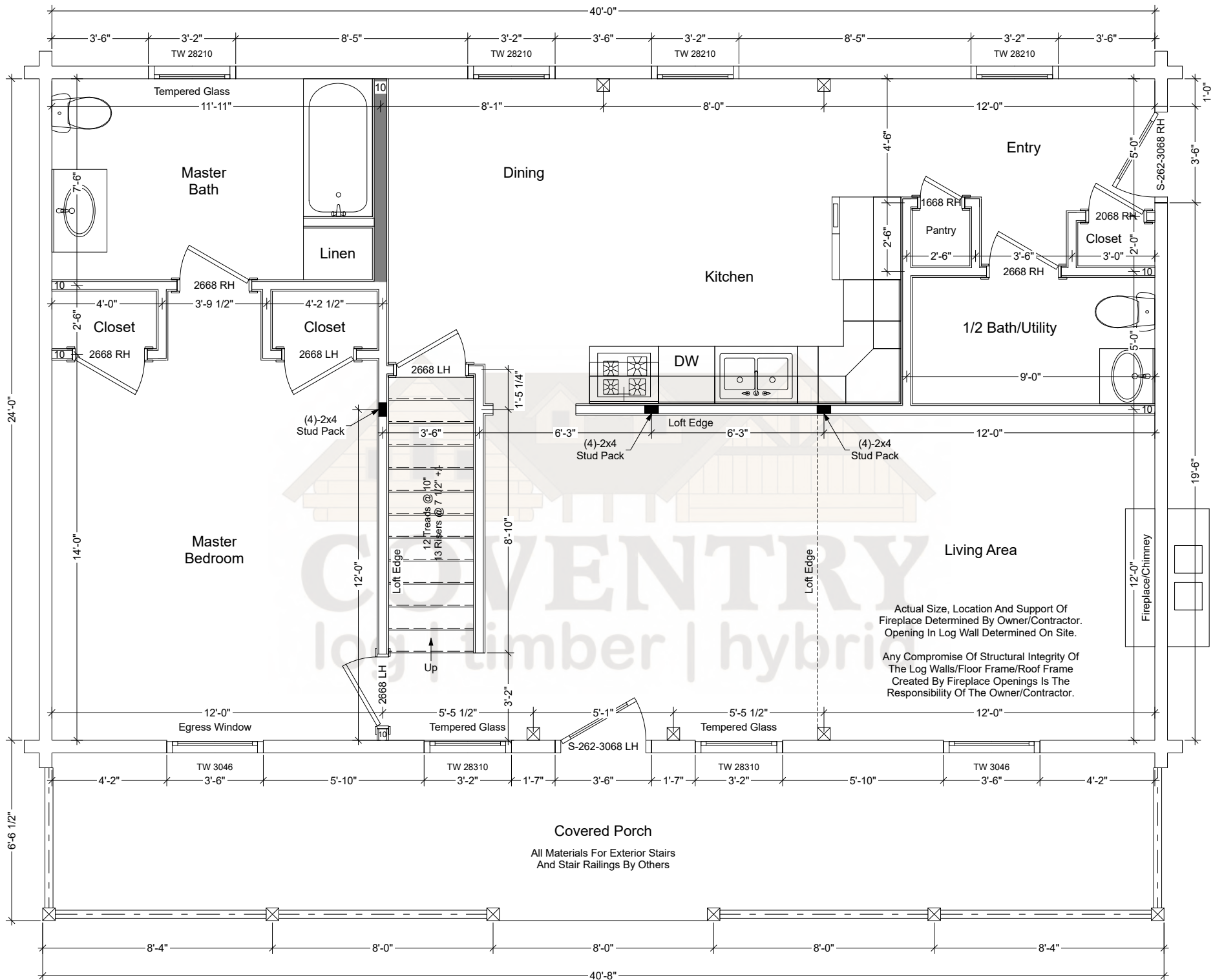
Wyoming First Floor Plan
